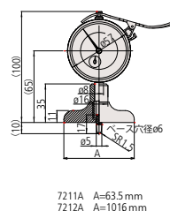
7211A A=63.5 mm 7212A A=101.6 mm
